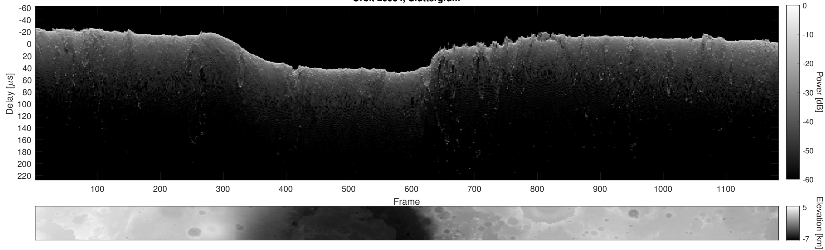
Orbit 20964, Cluttergram
