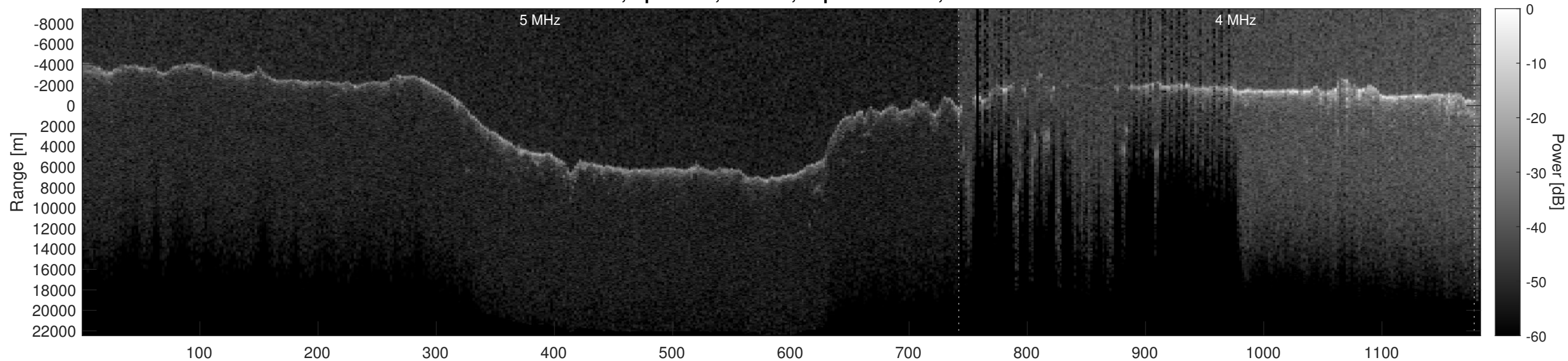
Orbit 20964, Optimized, Window, Depth-Corrected, Channel 2
