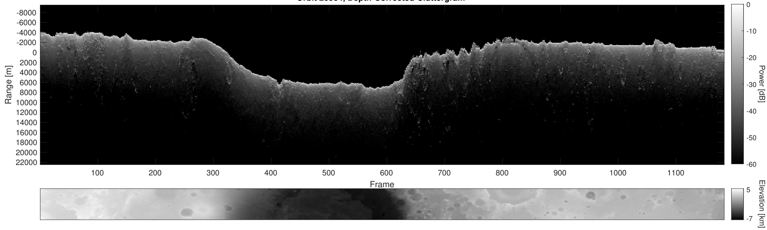
Orbit 20964, Depth-Corrected Cluttergram
