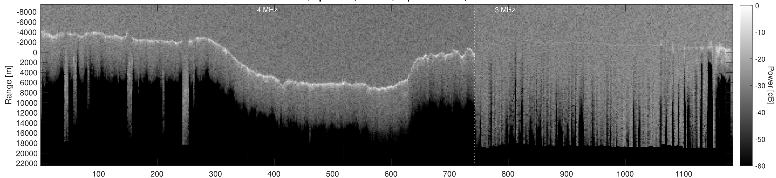
Orbit 20964, Depth-Corrected Cluttergram
