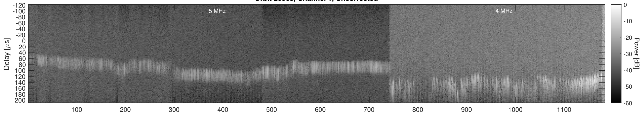
Orbit 20965, Window, Channel 1, Chapman
