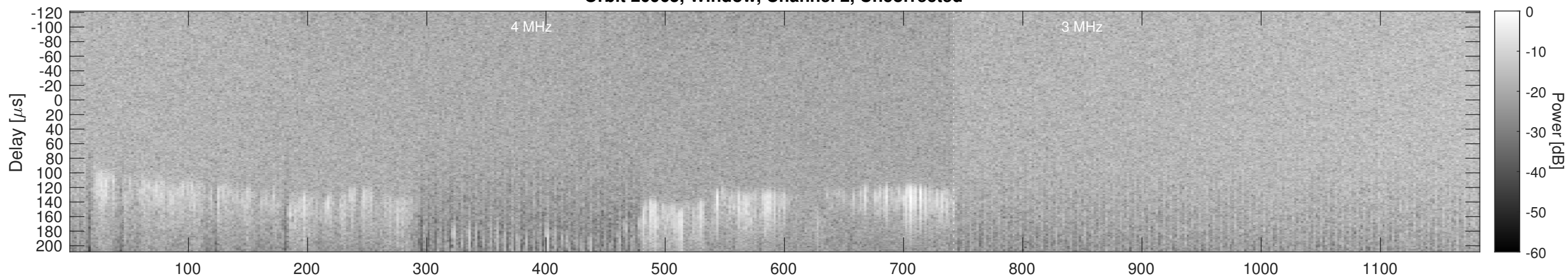
Orbit 20965, Window, Channel 2, Chapman
