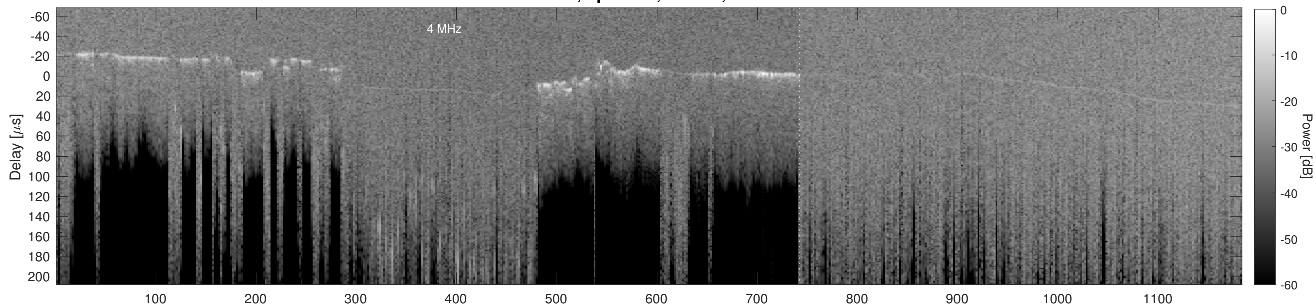
Orbit 20965, Cluttergram
