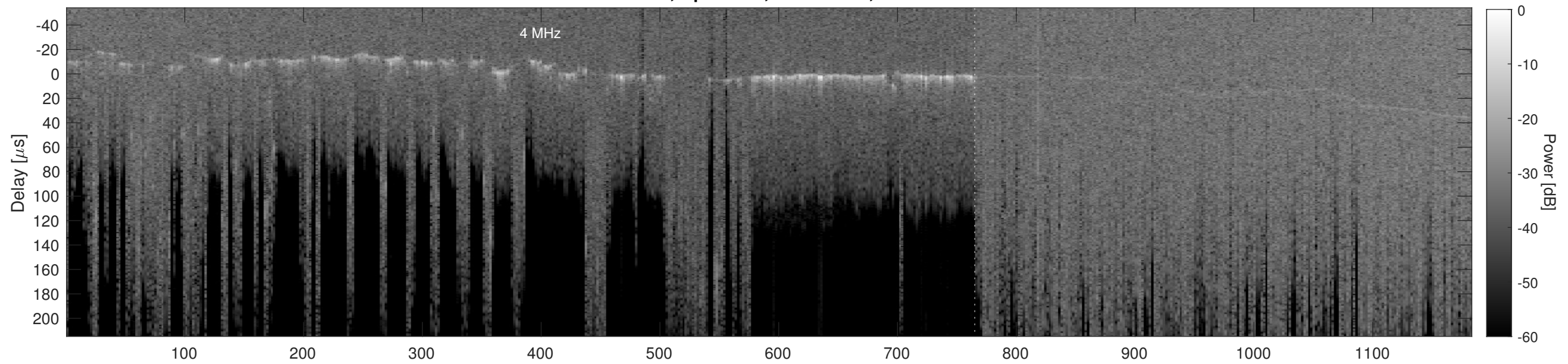
Orbit 20967, Cluttergram
