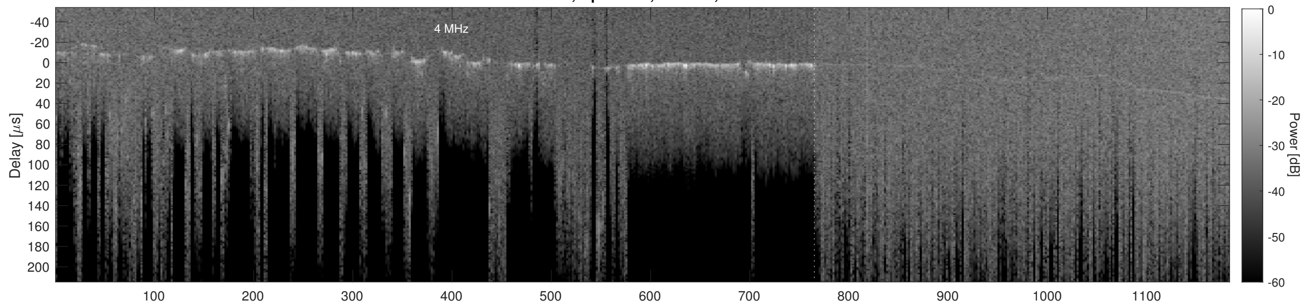
Orbit 20967, Cluttergram
