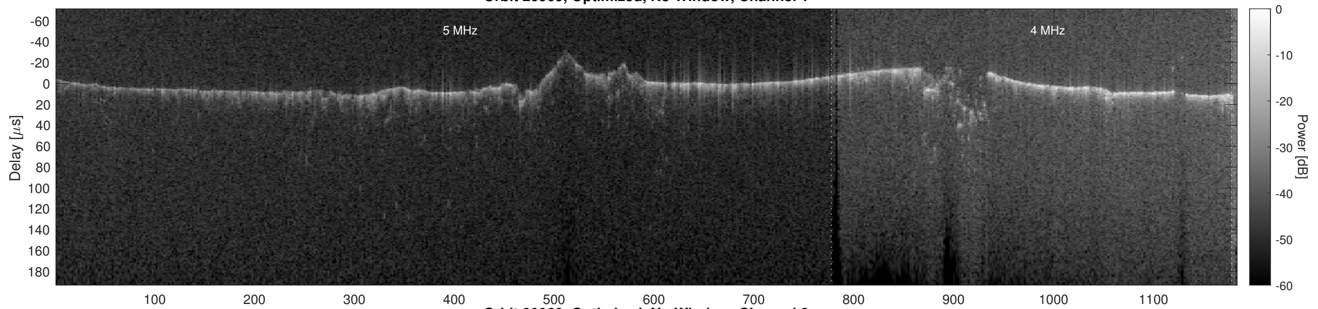
Orbit 20969, Optimized, No Window, Channel 2
