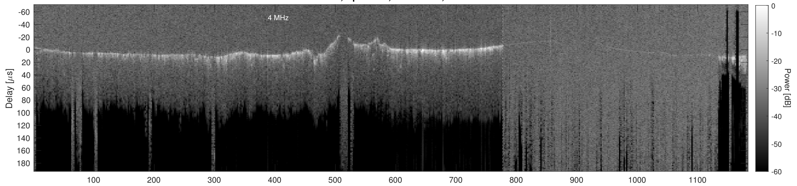
Orbit 20969, Cluttergram
