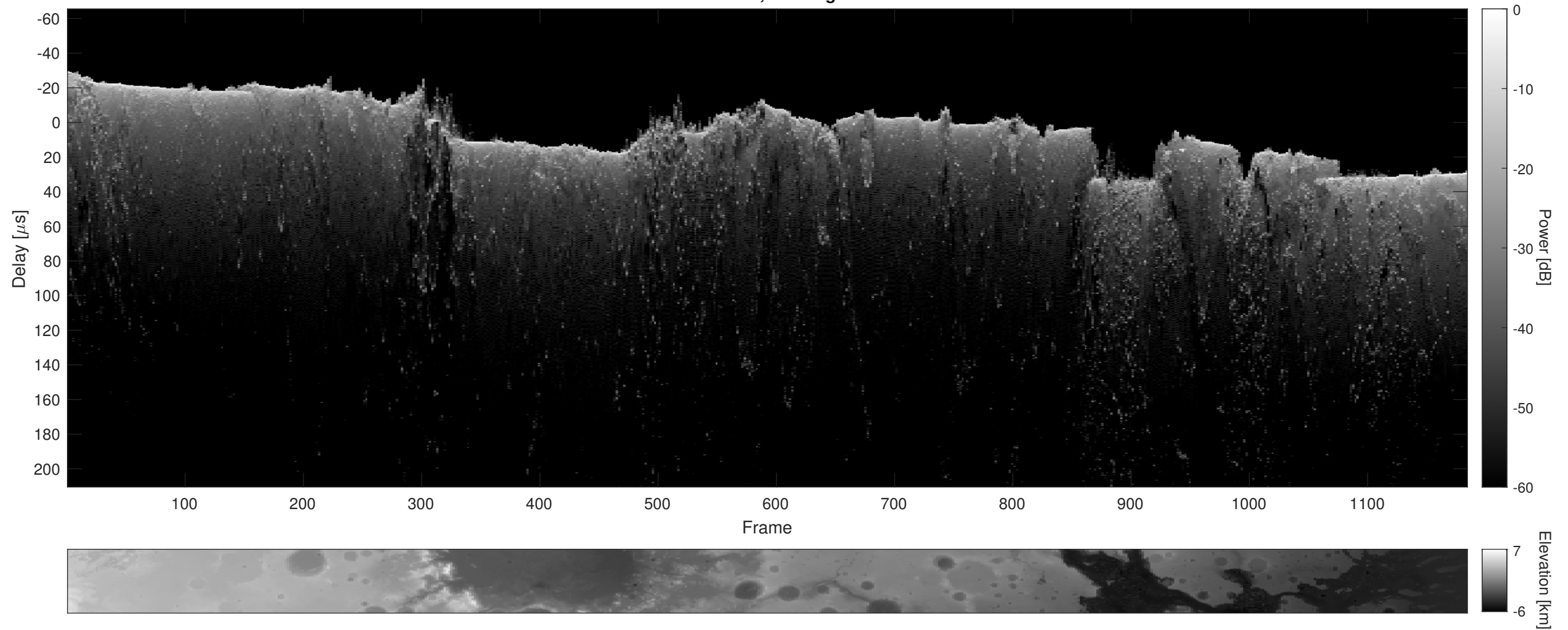
Orbit 20972, Cluttergram
