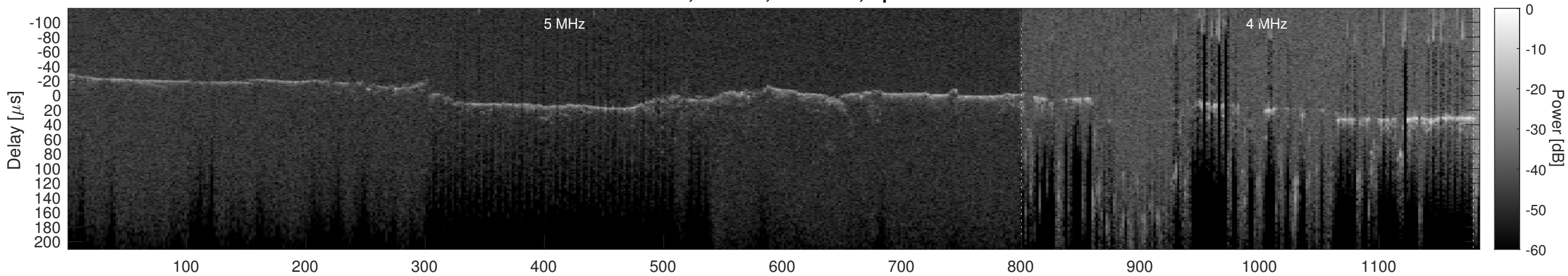
Orbit 20972, Cluttergram
