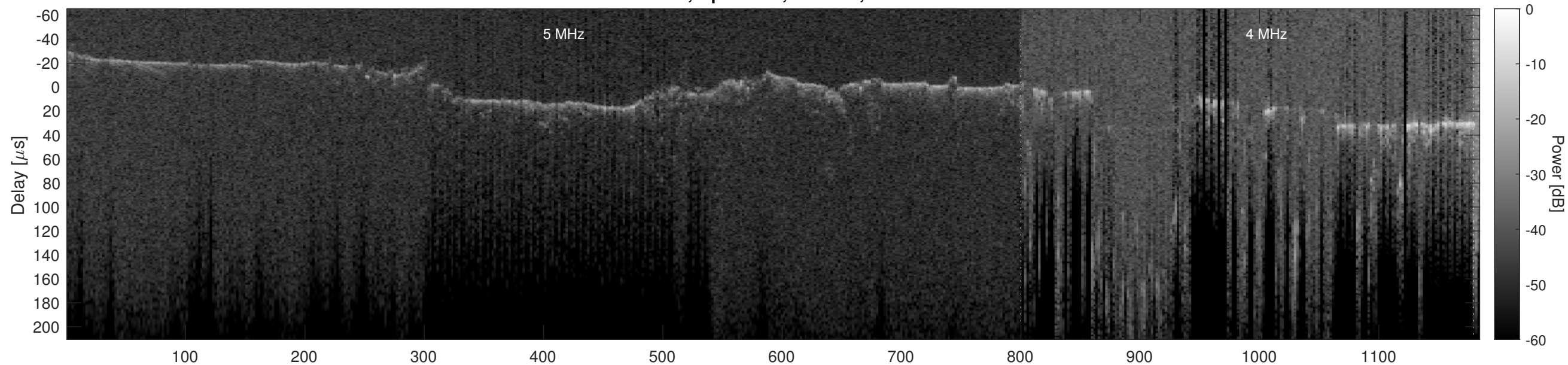
Orbit 20972, Optimized, Window, Channel 2
