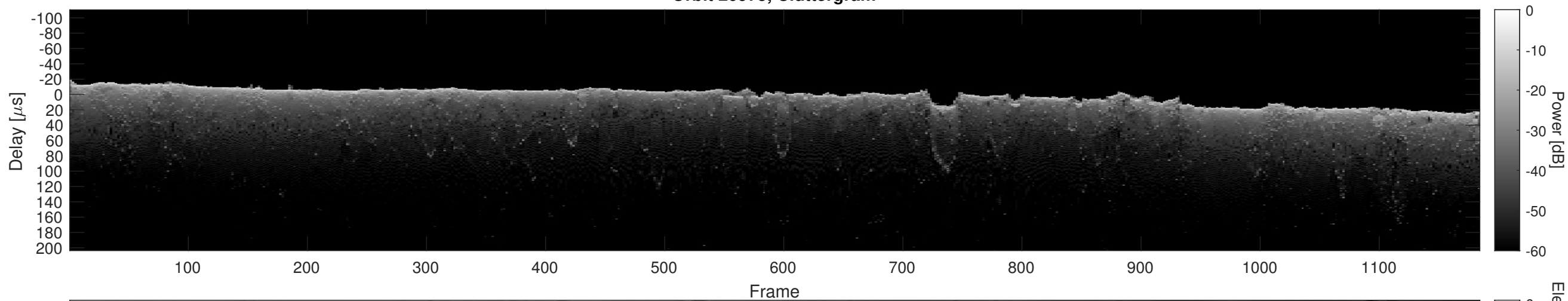
Orbit 20975, Cluttergram
