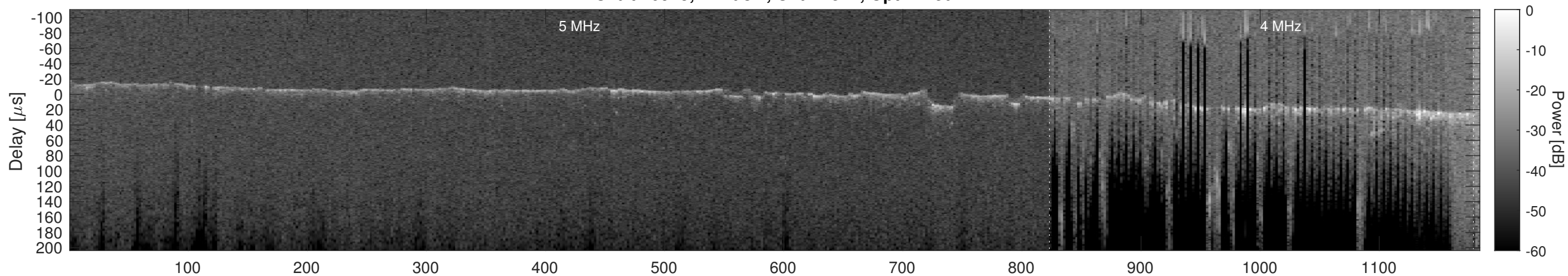
Orbit 20975, Cluttergram
