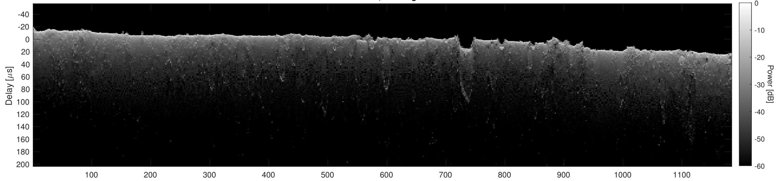
Orbit 20975, Cluttergram
