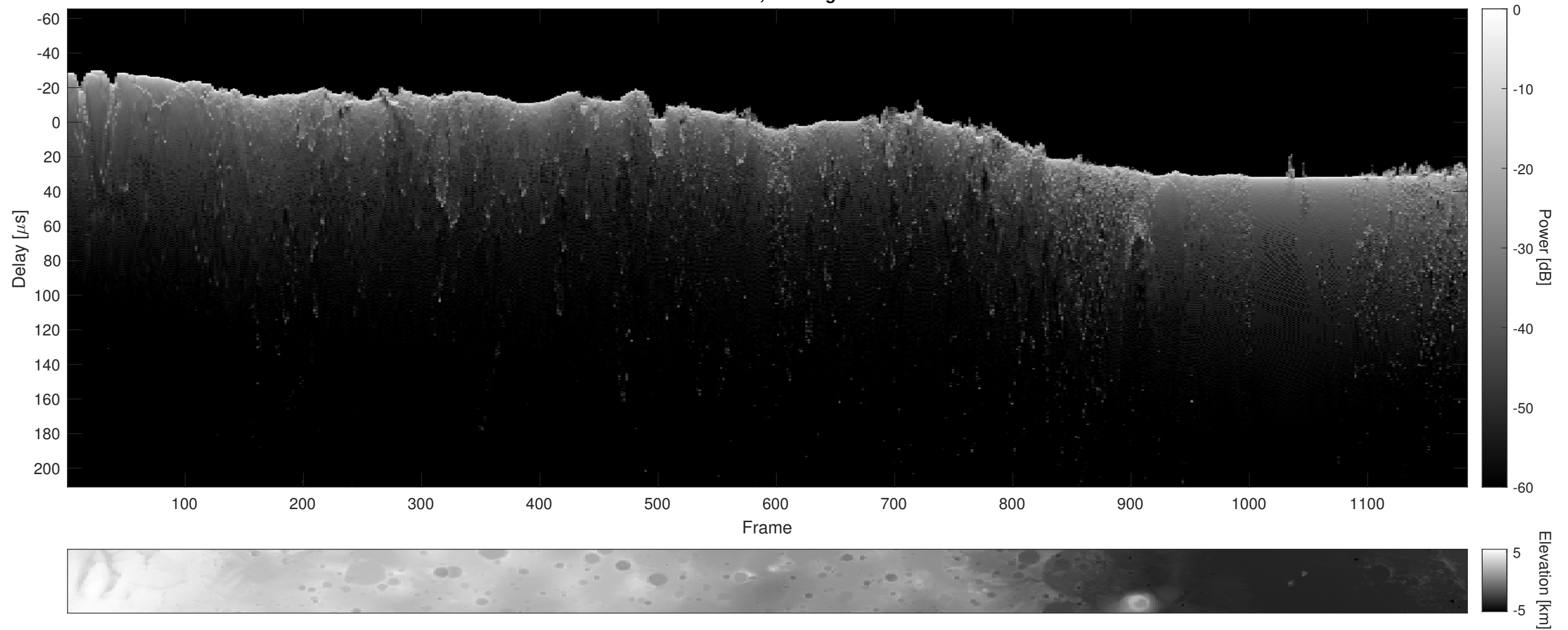
Orbit 20977, Cluttergram
