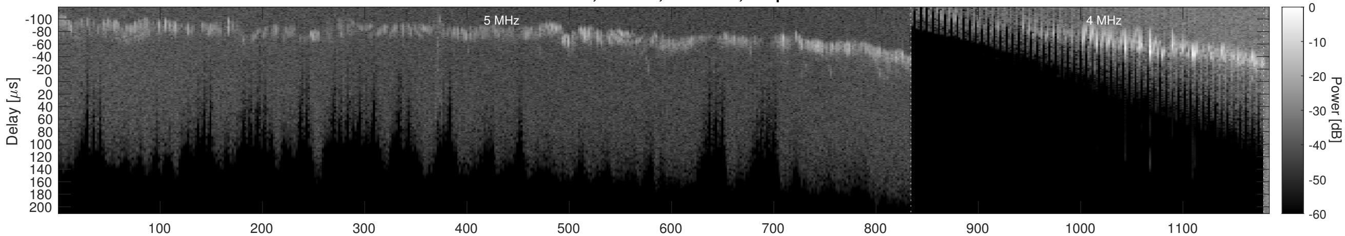
Orbit 20977, Window, Channel 1, Optimized
