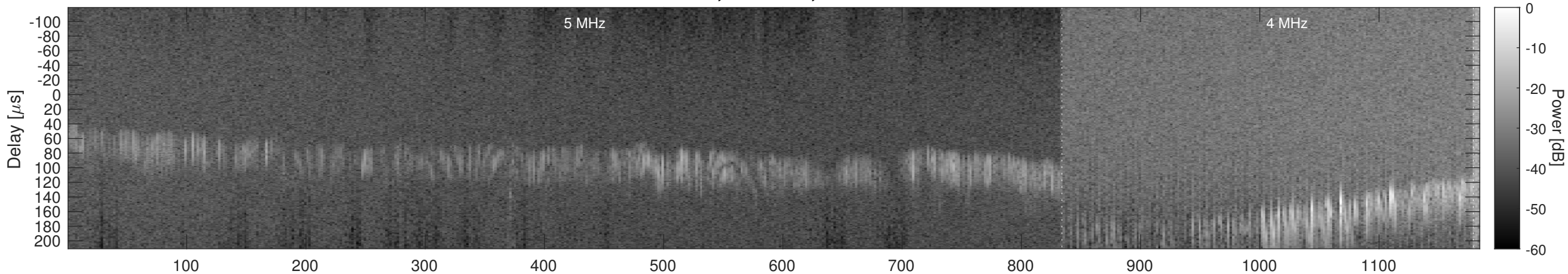
Orbit 20977, Window, Channel 1, Chapman
