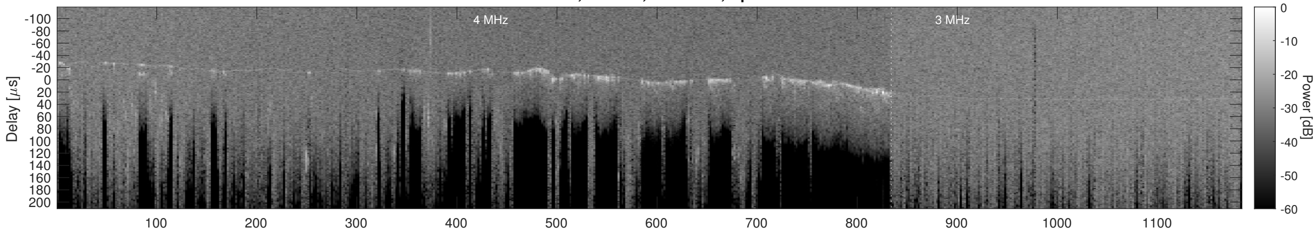
Orbit 20977, Cluttergram
