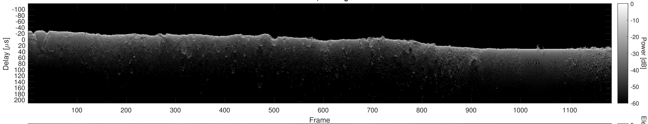
Orbit 20977, Cluttergram
