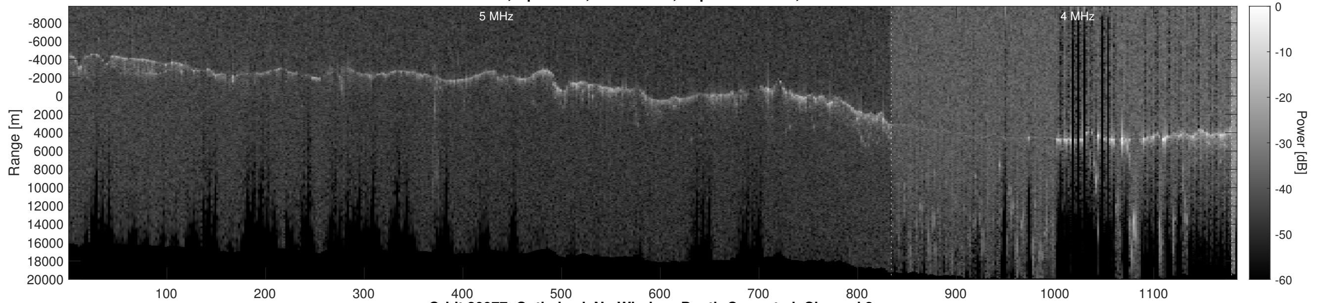
Orbit 20977, Optimized, No Window, Depth-Corrected, Channel 2
