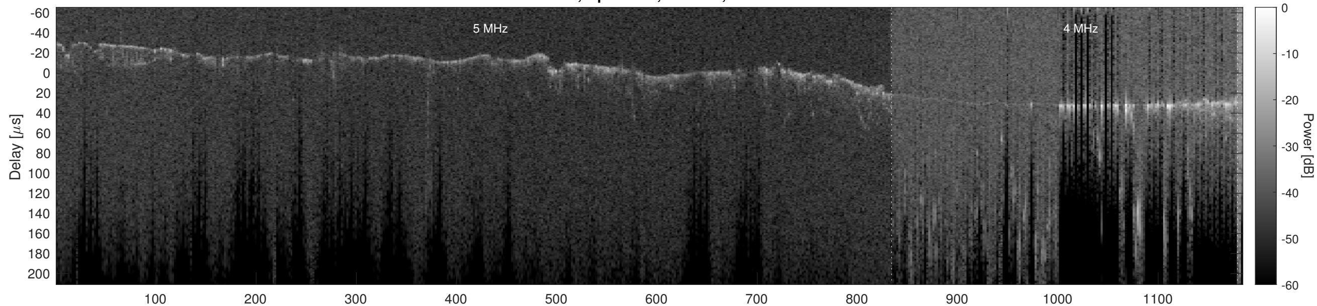
Orbit 20977, Optimized, Window, Channel 2
