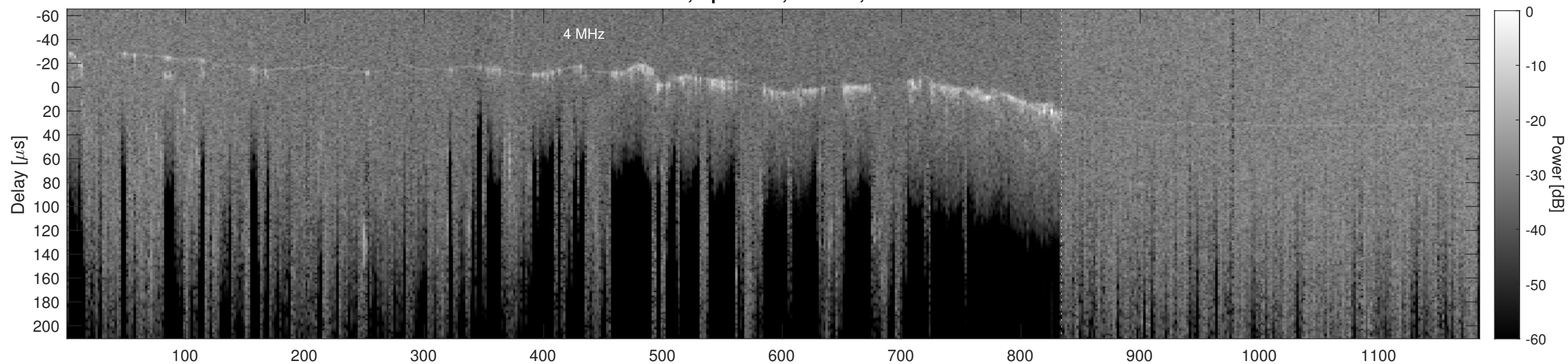
Orbit 20977, Cluttergram
