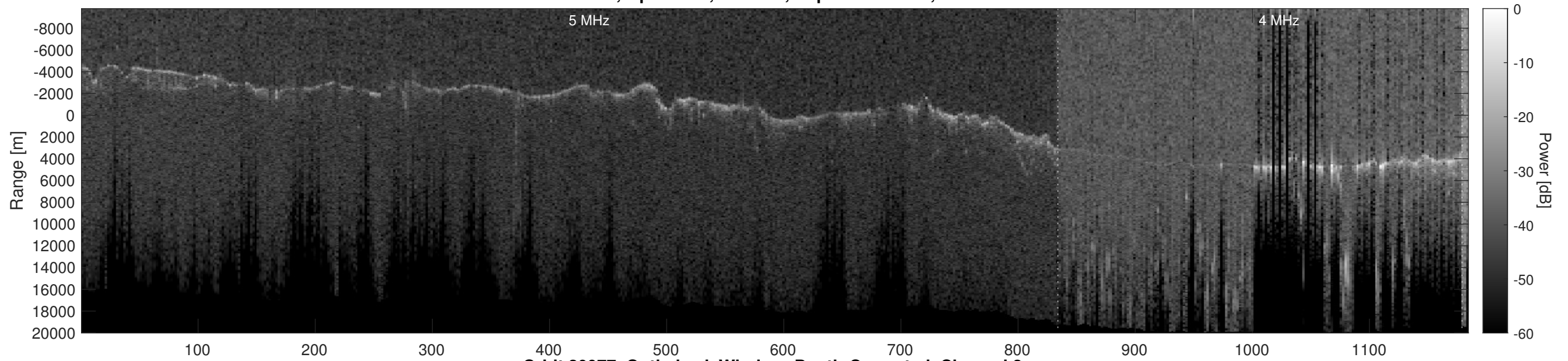
Orbit 20977, Optimized, Window, Depth-Corrected, Channel 2
