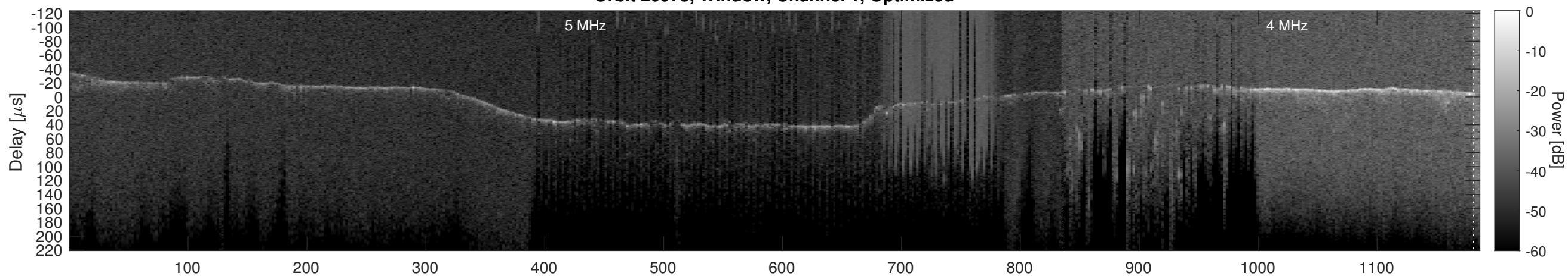
Orbit 20978, Cluttergram
