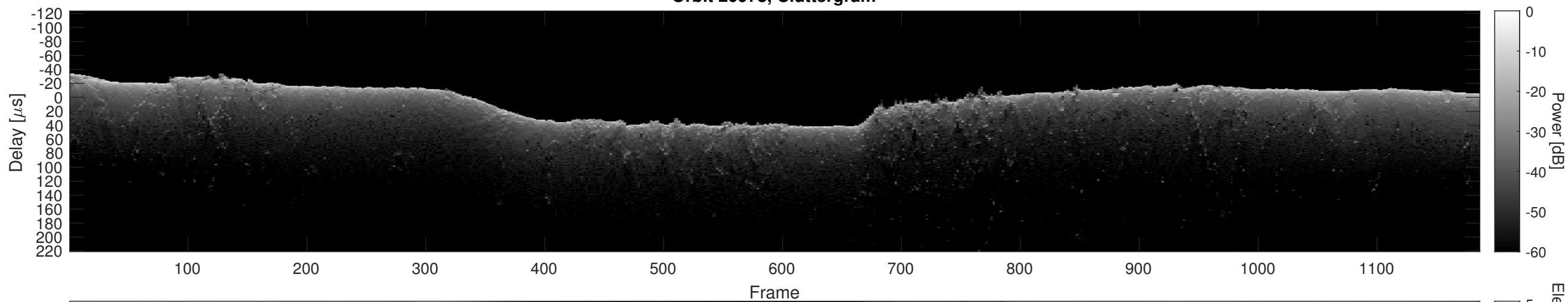
Orbit 20978, Cluttergram
