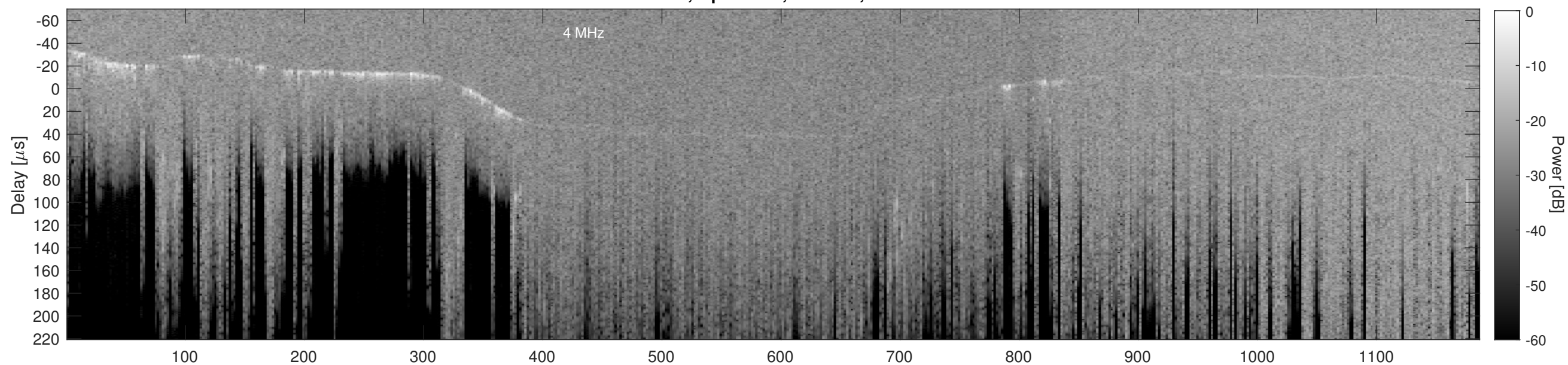
Orbit 20978, Cluttergram
