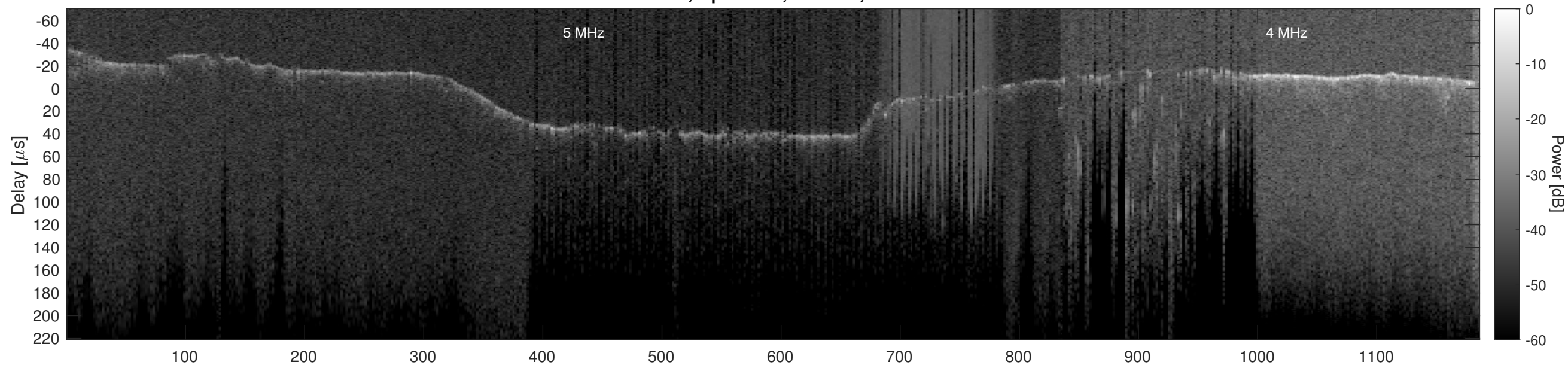
Orbit 20978, Optimized, Window, Channel 2
