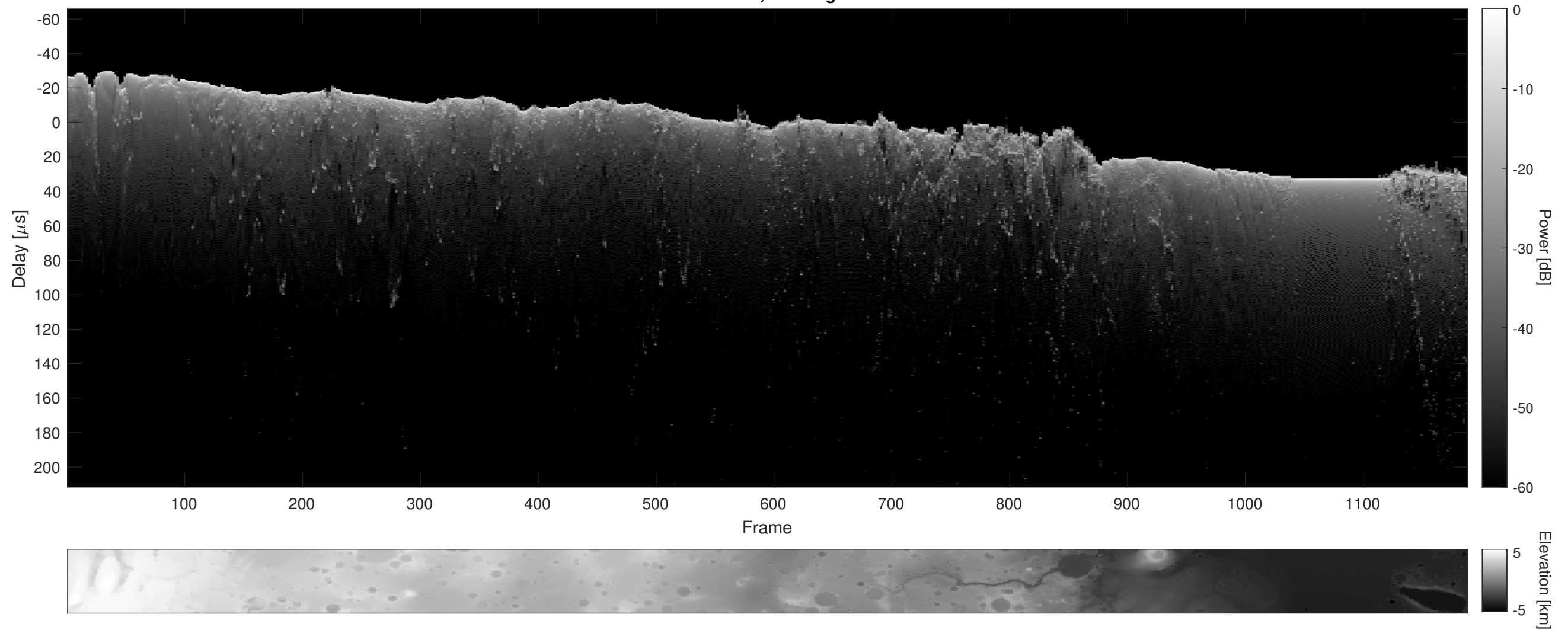
Orbit 20984, Cluttergram
