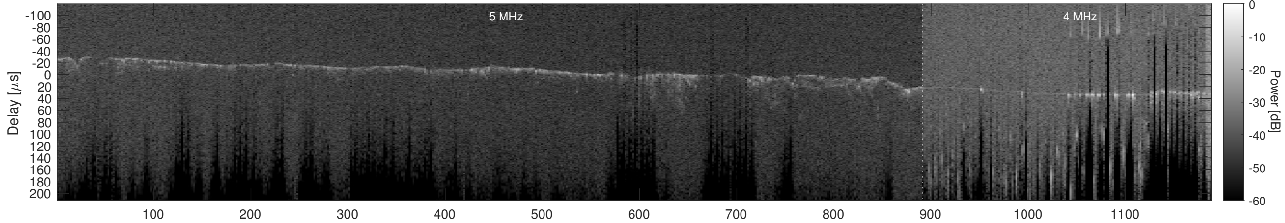
Orbit 20984, Cluttergram
