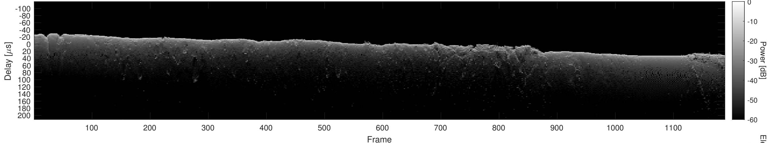
Orbit 20984, Cluttergram
