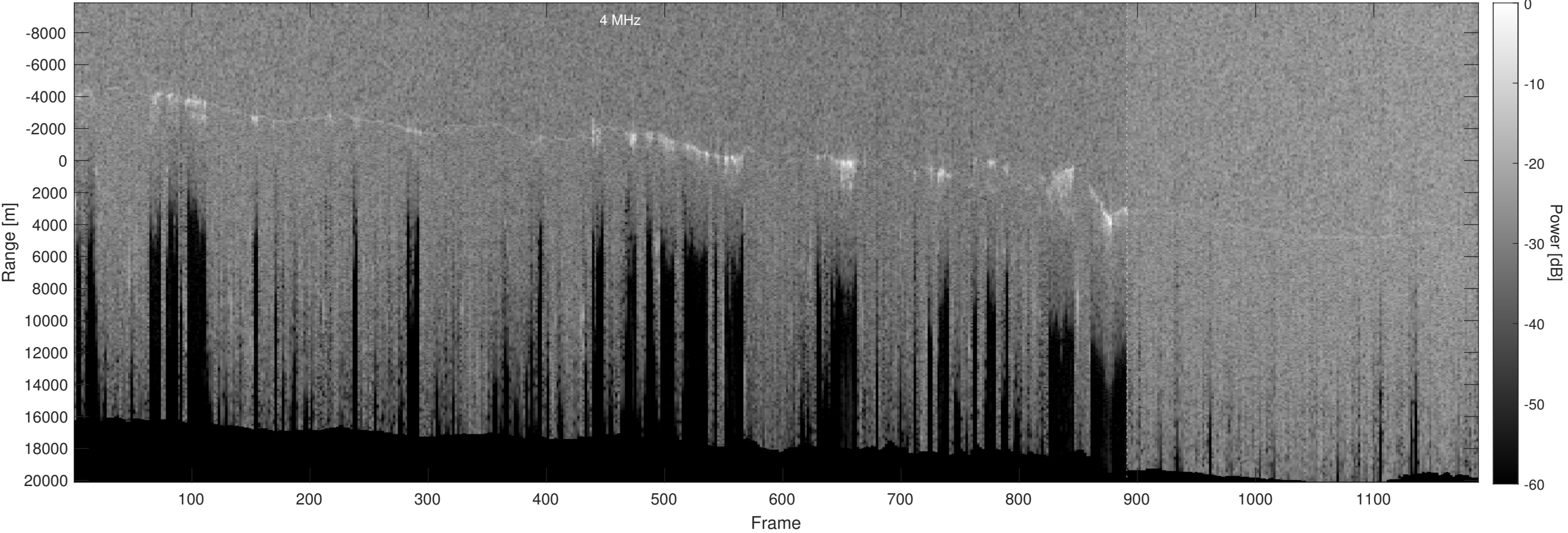
Orbit 20984, Optimized, No Window, Depth-Corrected, Channel 2
