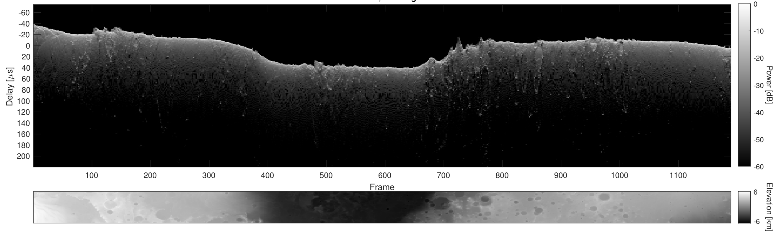
Orbit 20985, Cluttergram
