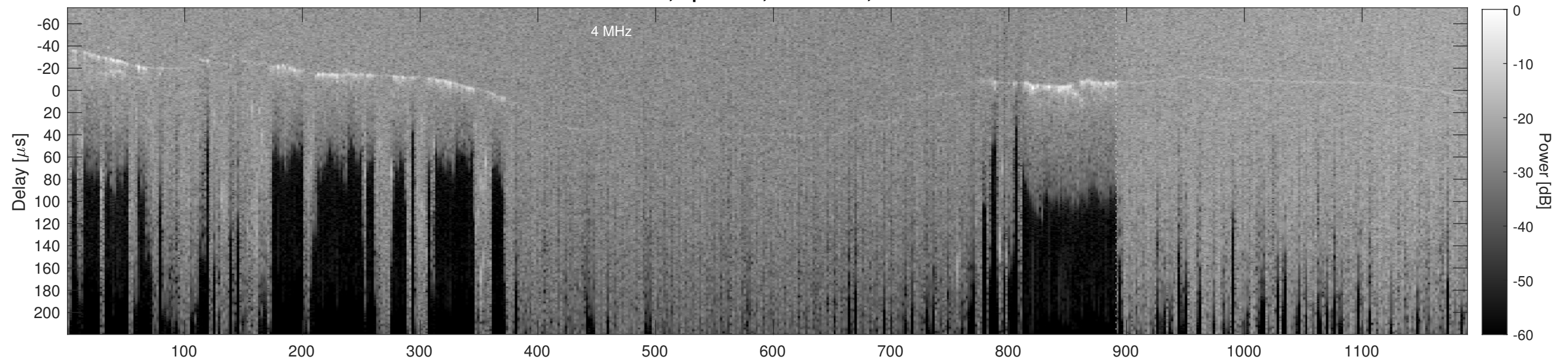
Orbit 20985, Cluttergram
