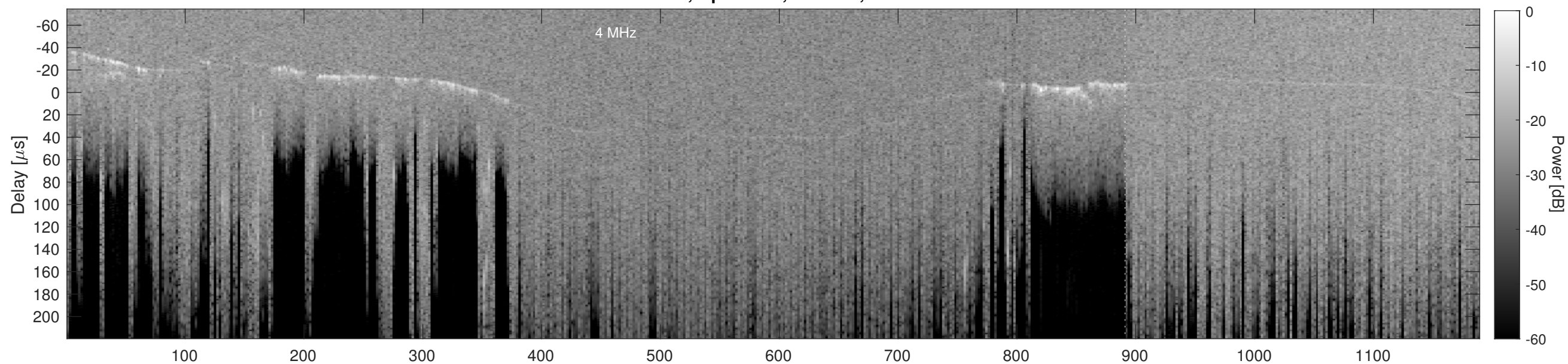
Orbit 20985, Cluttergram
