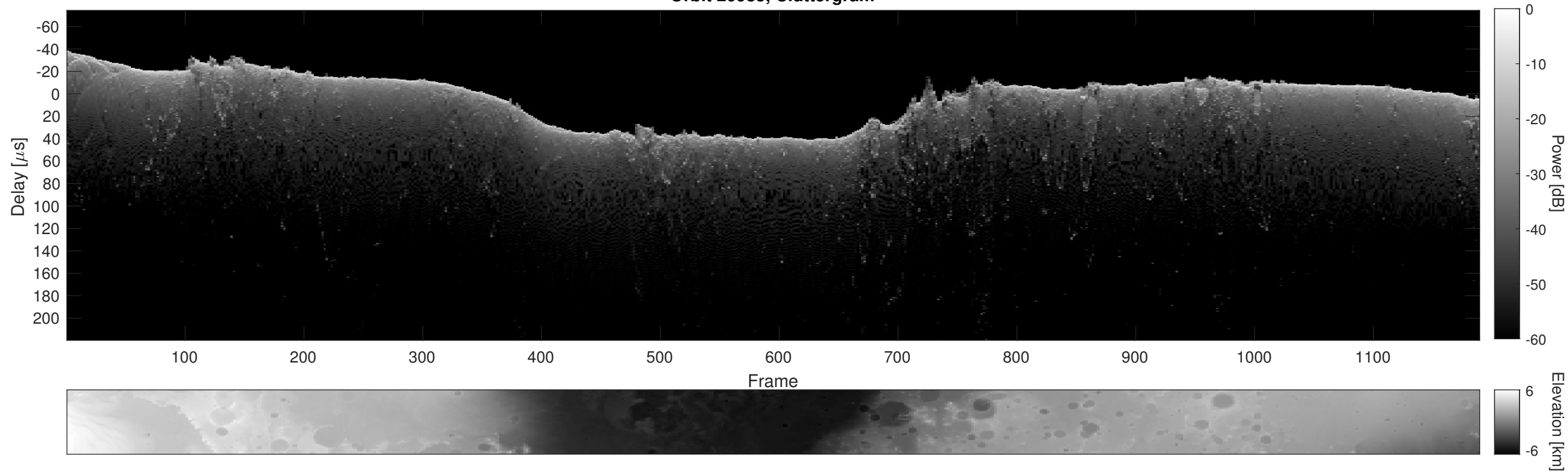
Orbit 20985, Cluttergram
