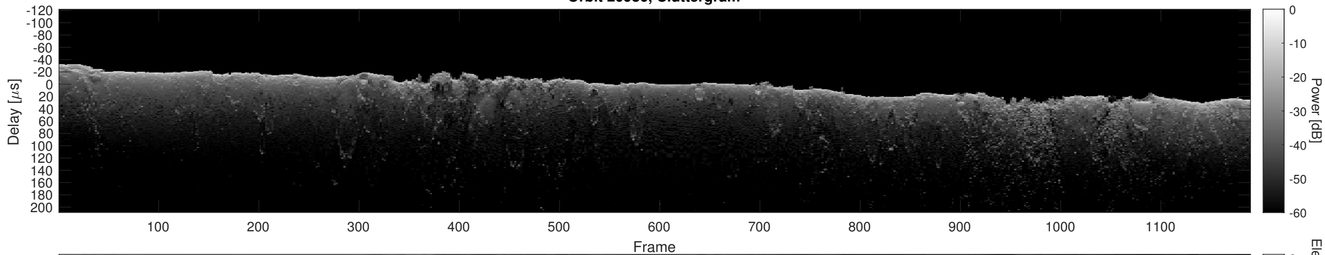
Orbit 20986, Cluttergram
