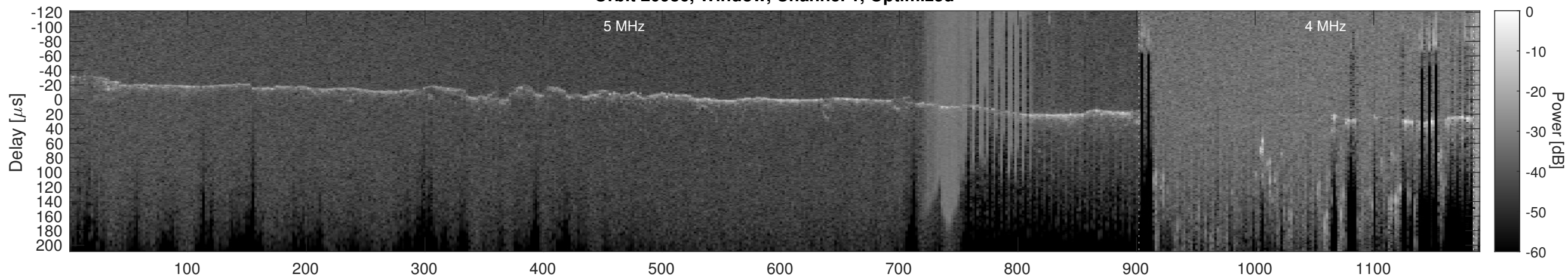
Orbit 20986, Cluttergram
