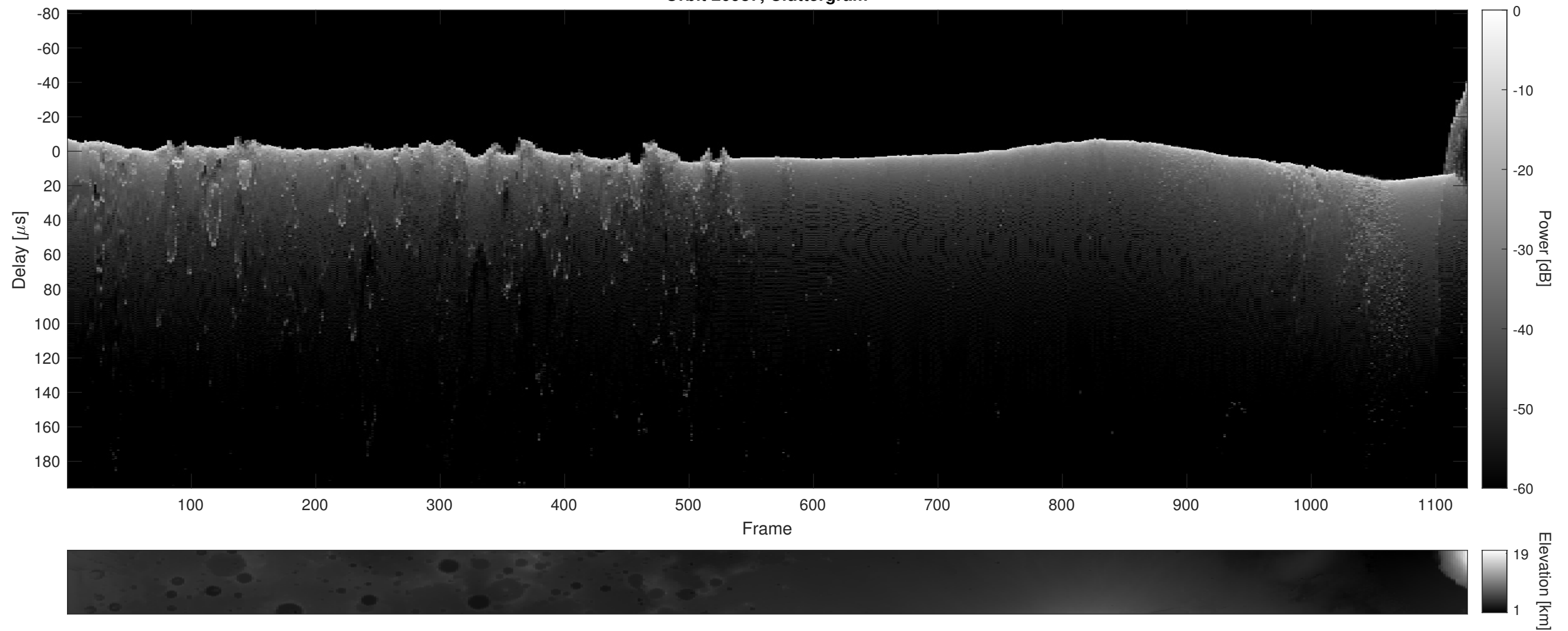
Orbit 20987, Cluttergram
