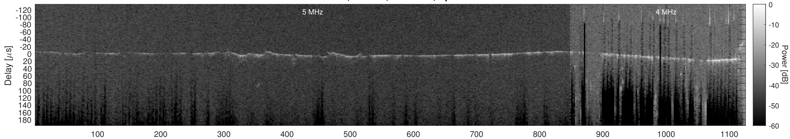
Orbit 20987, Cluttergram
