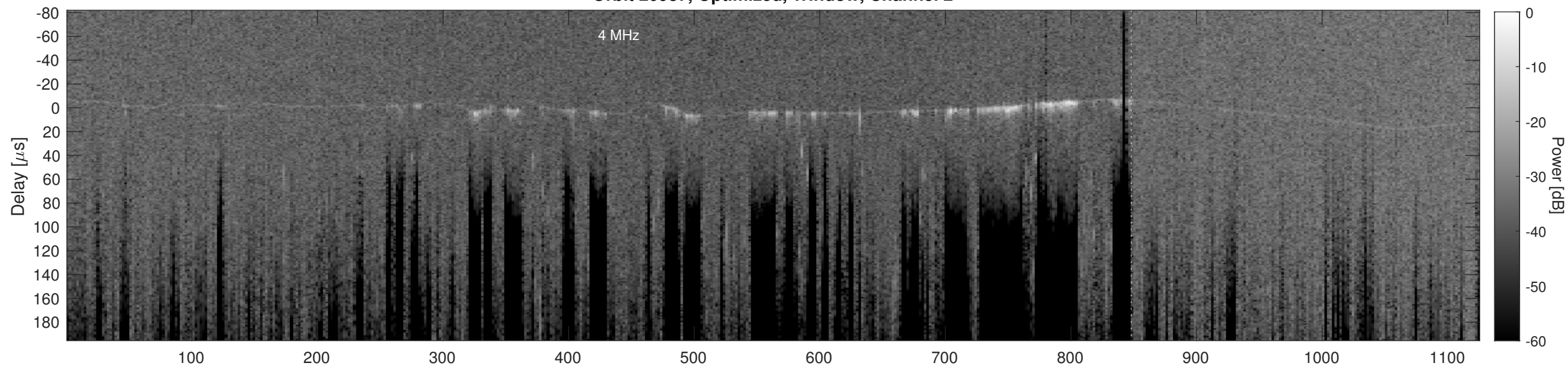
Orbit 20987, Cluttergram
