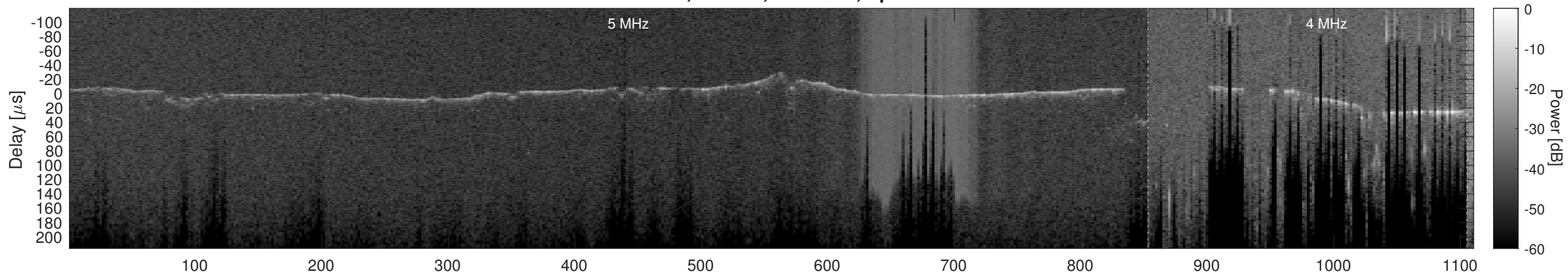
Orbit 20990, Cluttergram
