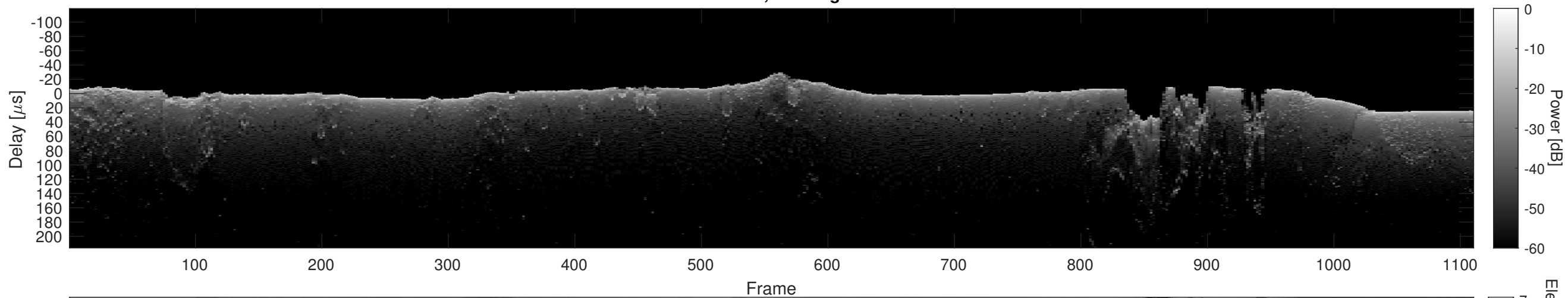
Orbit 20990, Cluttergram
