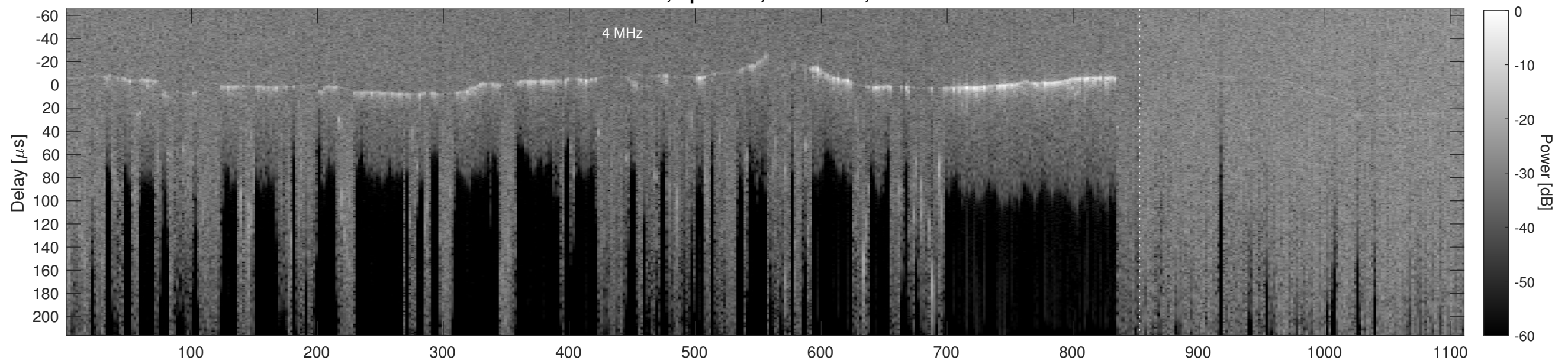
Orbit 20990, Cluttergram
