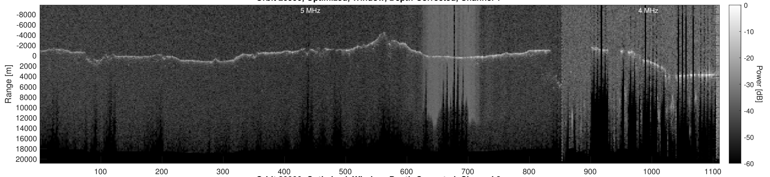
Orbit 20990, Optimized, Window, Depth-Corrected, Channel 2
