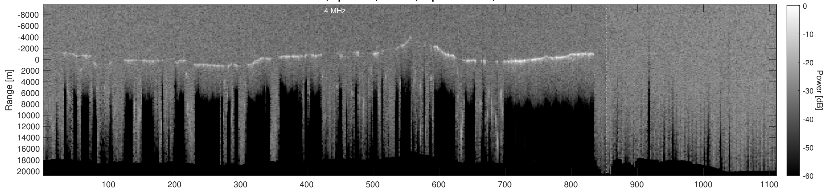
Orbit 20990, Depth-Corrected Cluttergram
