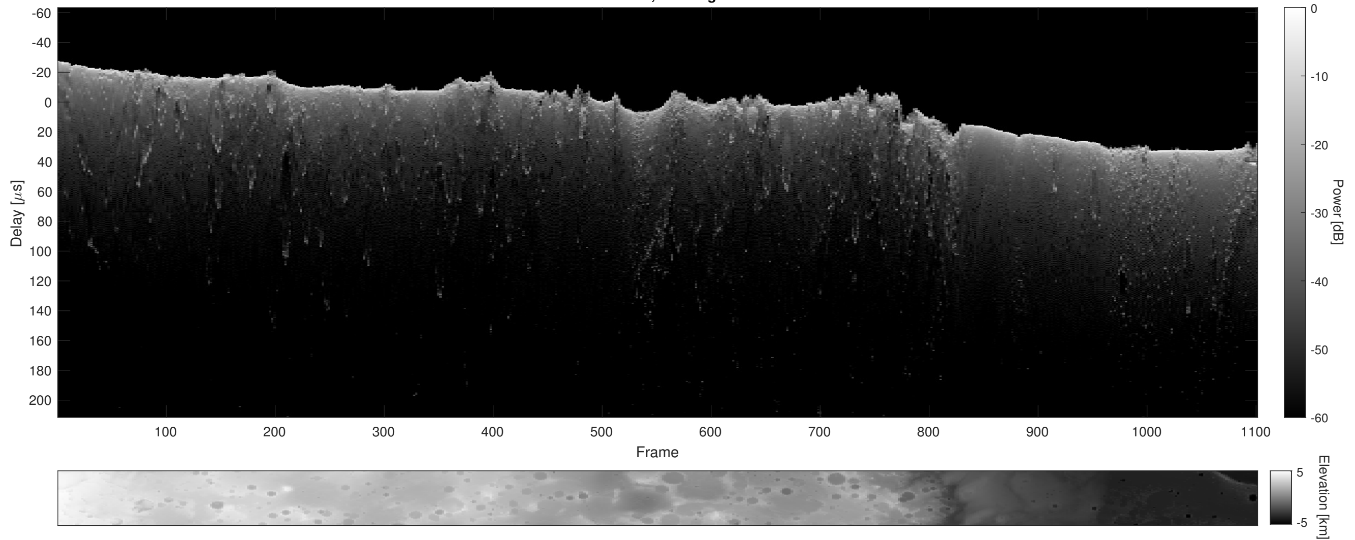
Orbit 20991, Cluttergram
