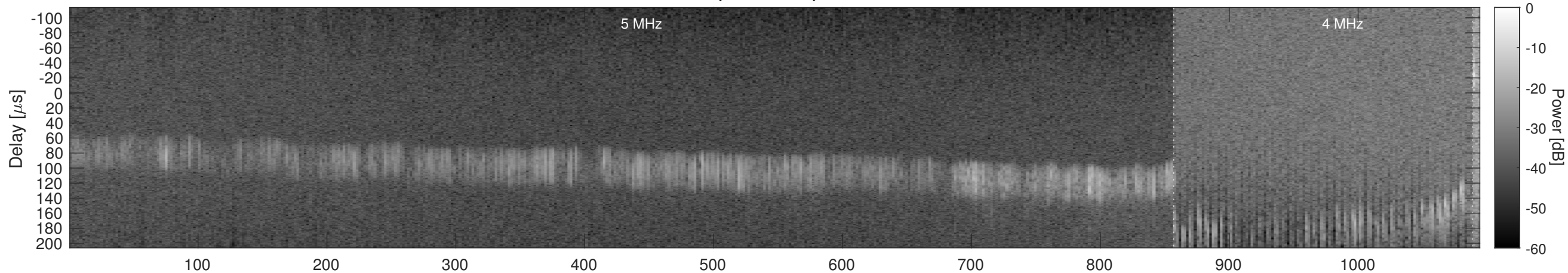
Orbit 20993, Window, Channel 1, Chapman
