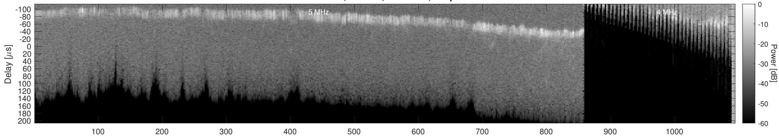
Orbit 20993, Window, Channel 1, Optimized
