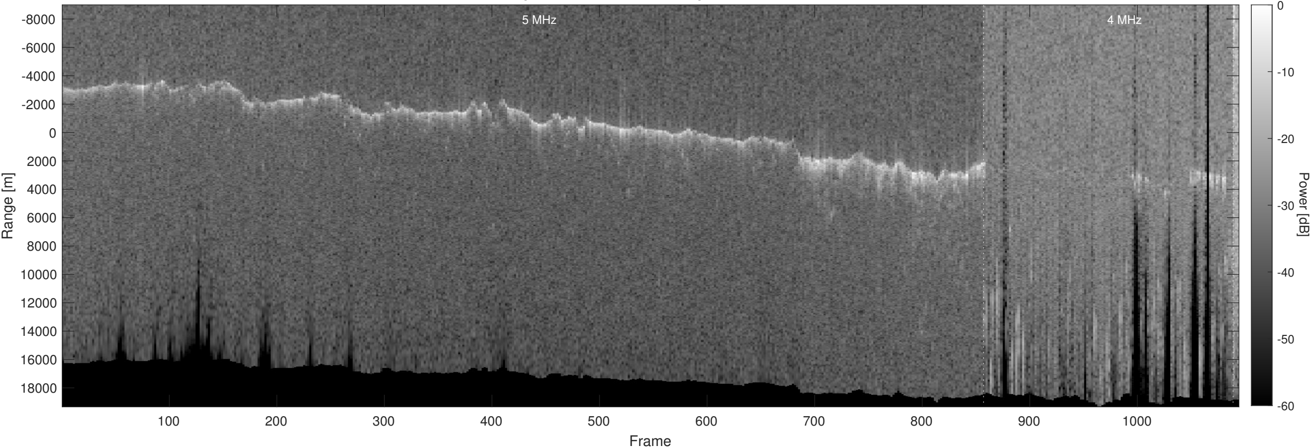
Orbit 20993, Optimized, No Window, Depth-Corrected, Channel 2
