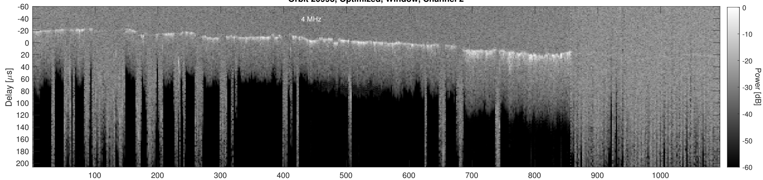
Orbit 20993, Cluttergram
