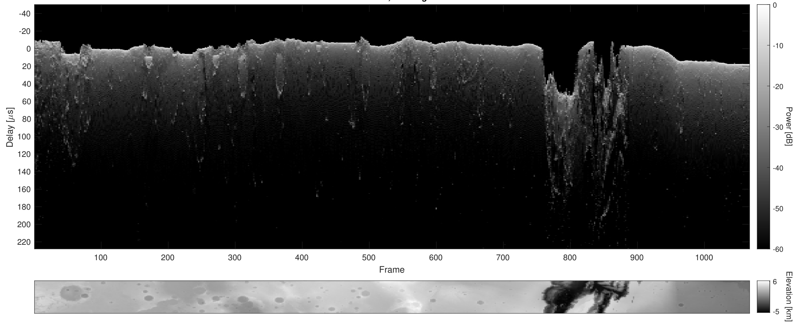
Orbit 20997, Cluttergram
