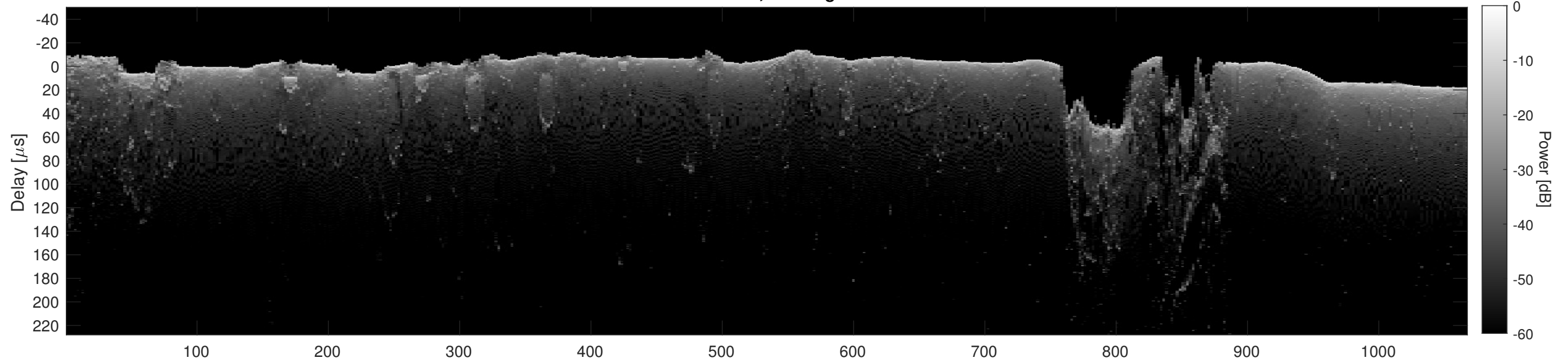
Orbit 20997, Cluttergram
