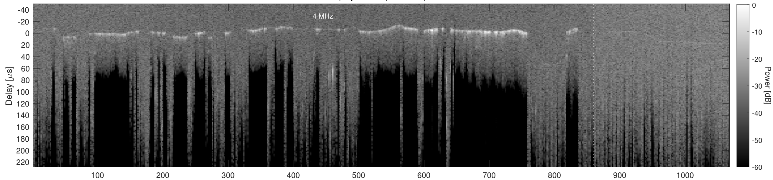
Orbit 20997, Cluttergram
