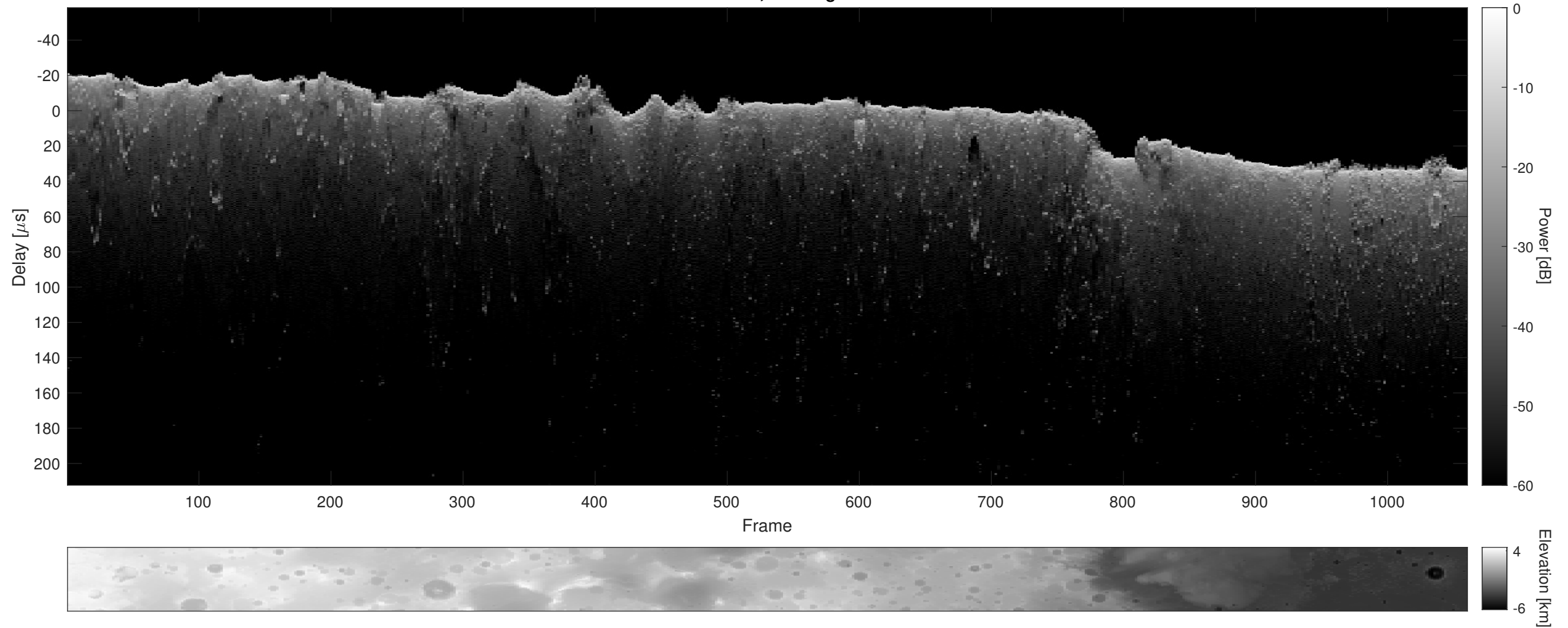
Orbit 20998, Cluttergram
