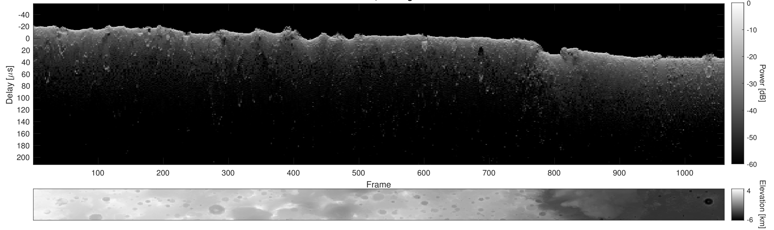
Orbit 20998, Cluttergram
