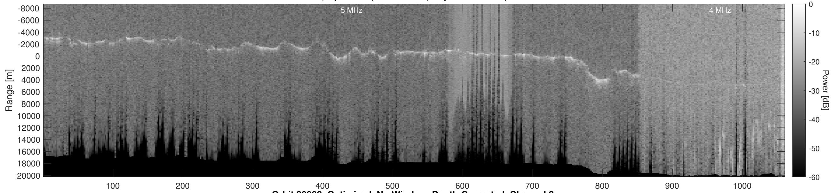
Orbit 20998, Optimized, No Window, Depth-Corrected, Channel 2
