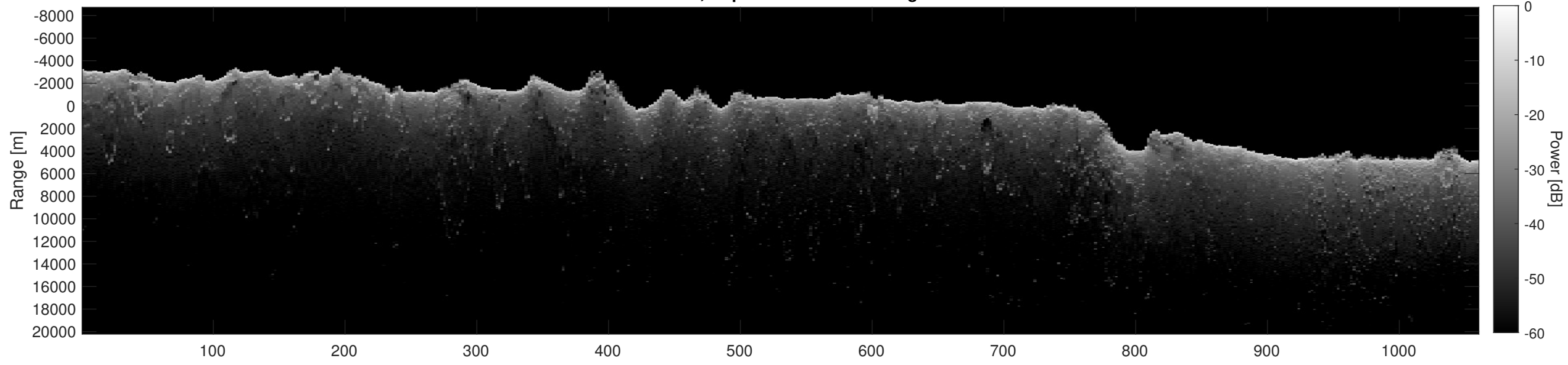
Orbit 20998, Depth-Corrected Cluttergram
