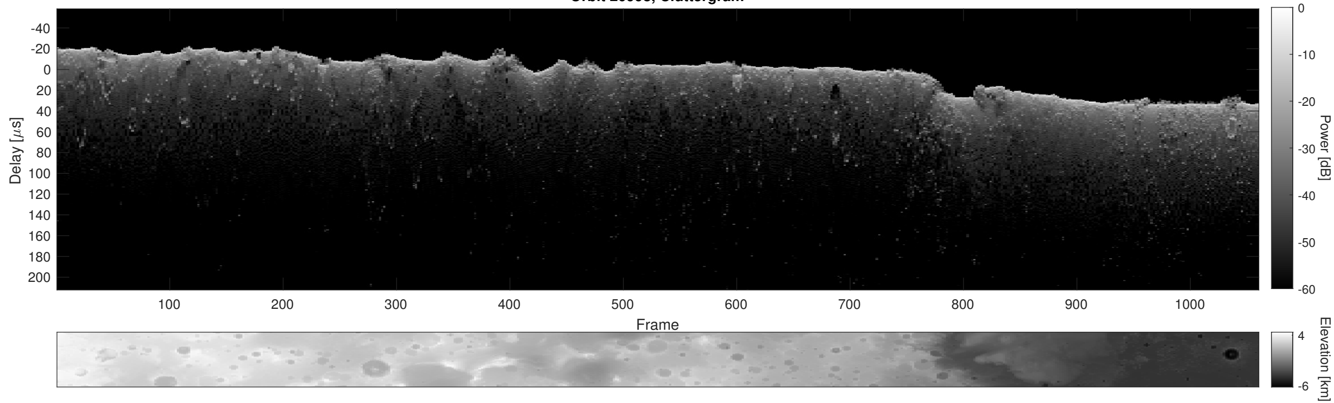
Orbit 20998, Cluttergram
