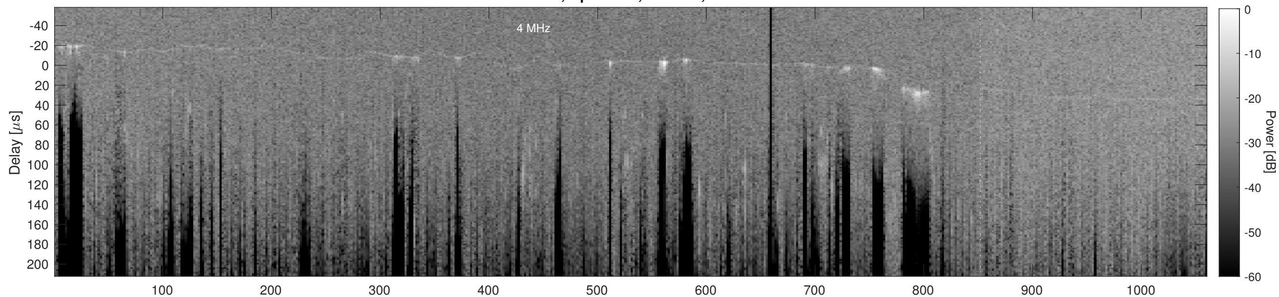
Orbit 20998, Cluttergram
