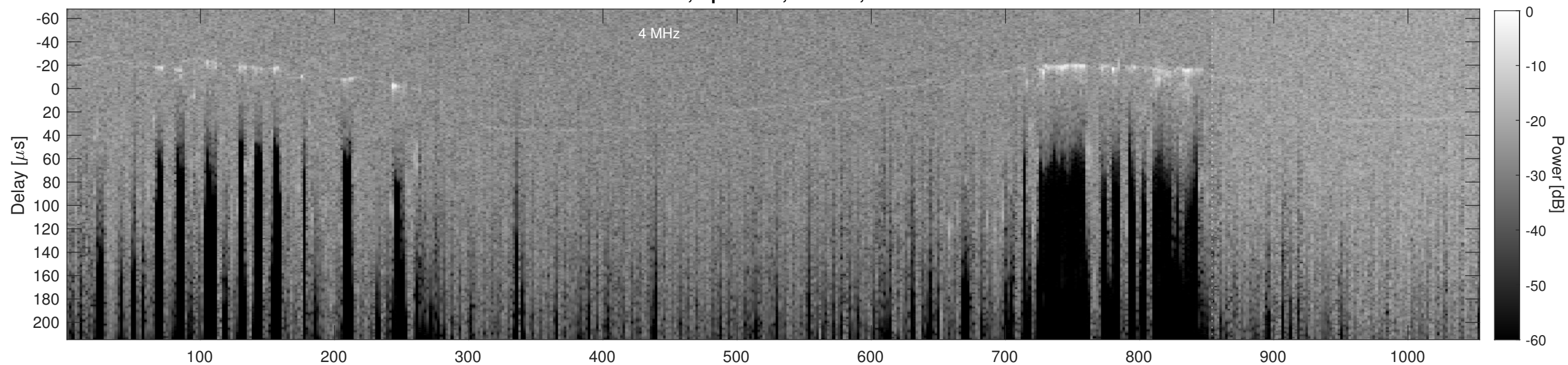
Orbit 20999, Cluttergram
