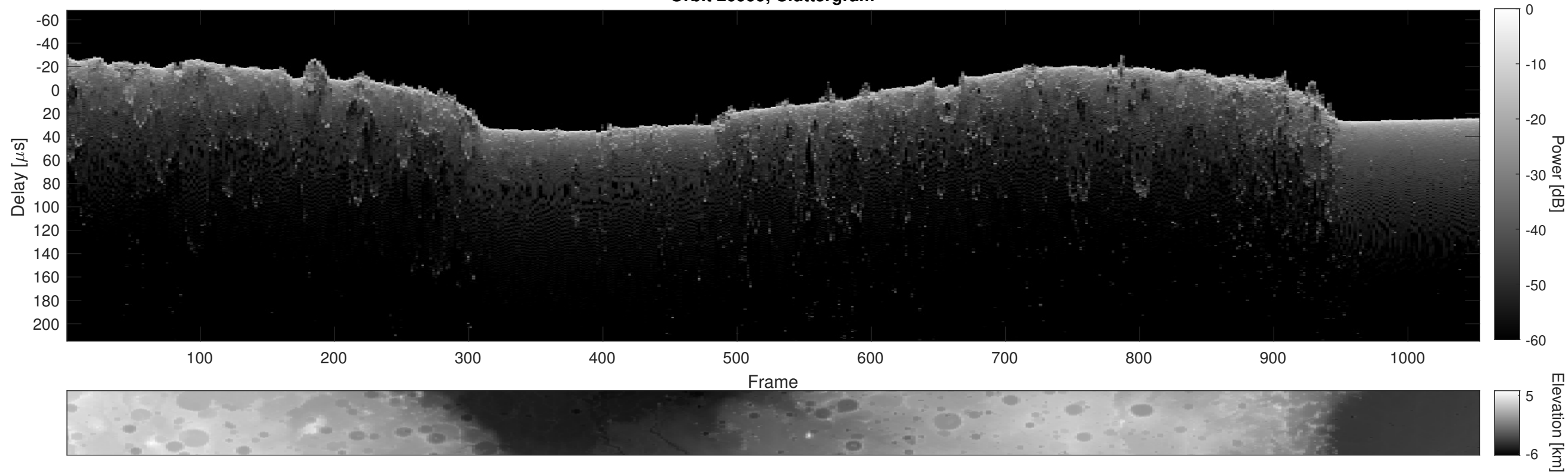
Orbit 20999, Cluttergram
