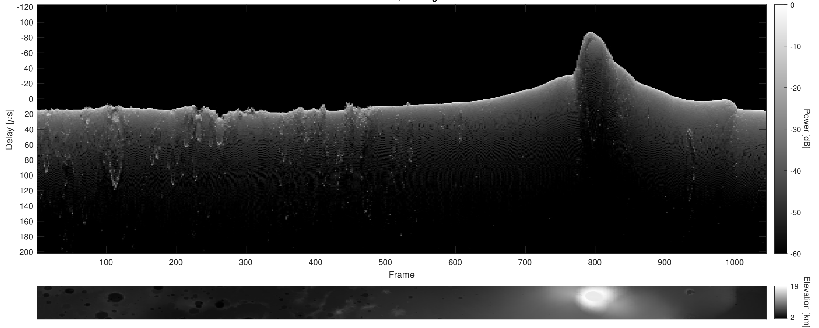
Orbit 21001, Cluttergram
