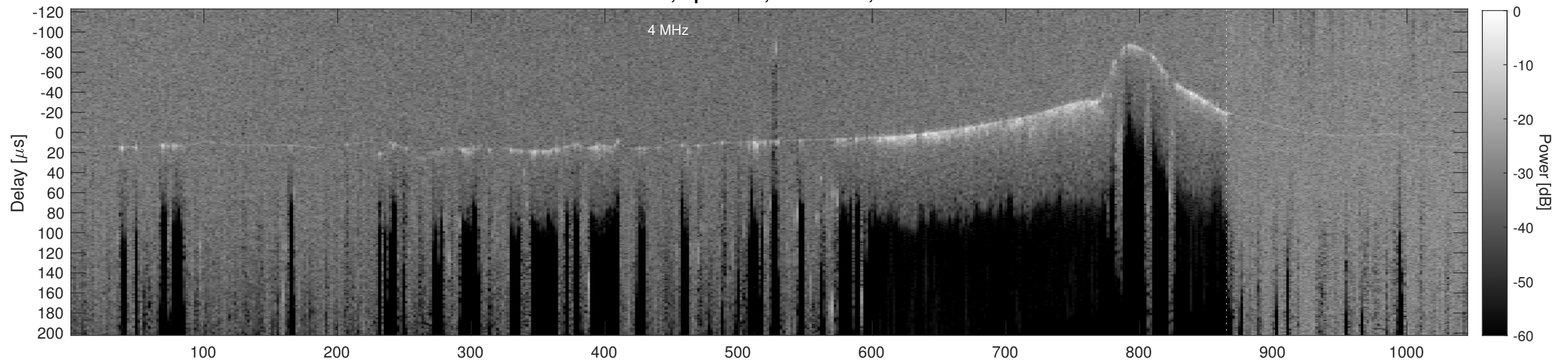
Orbit 21001, Cluttergram
