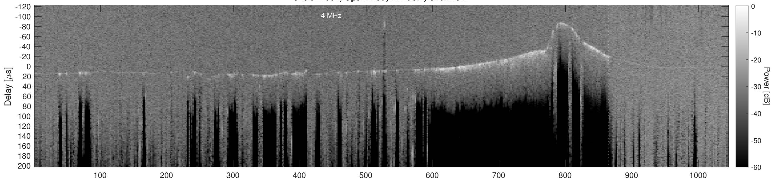
Orbit 21001, Cluttergram
