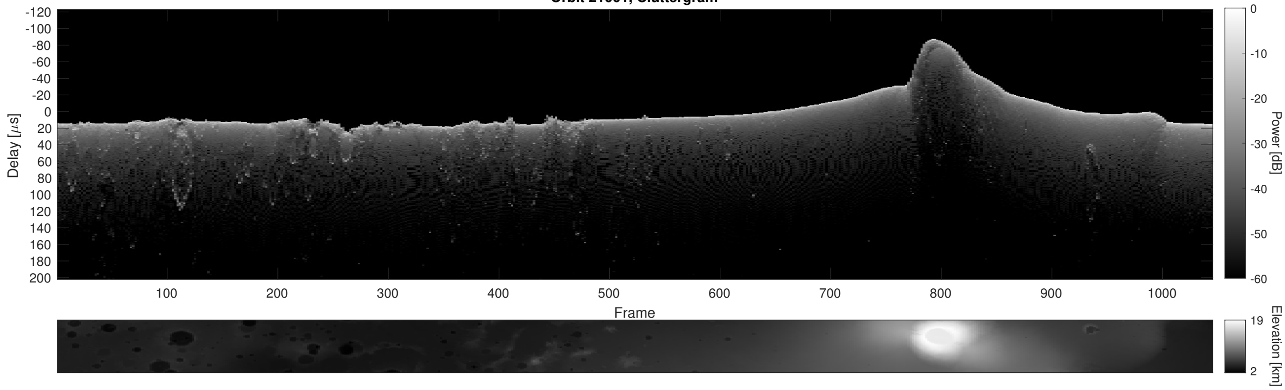
Orbit 21001, Cluttergram
