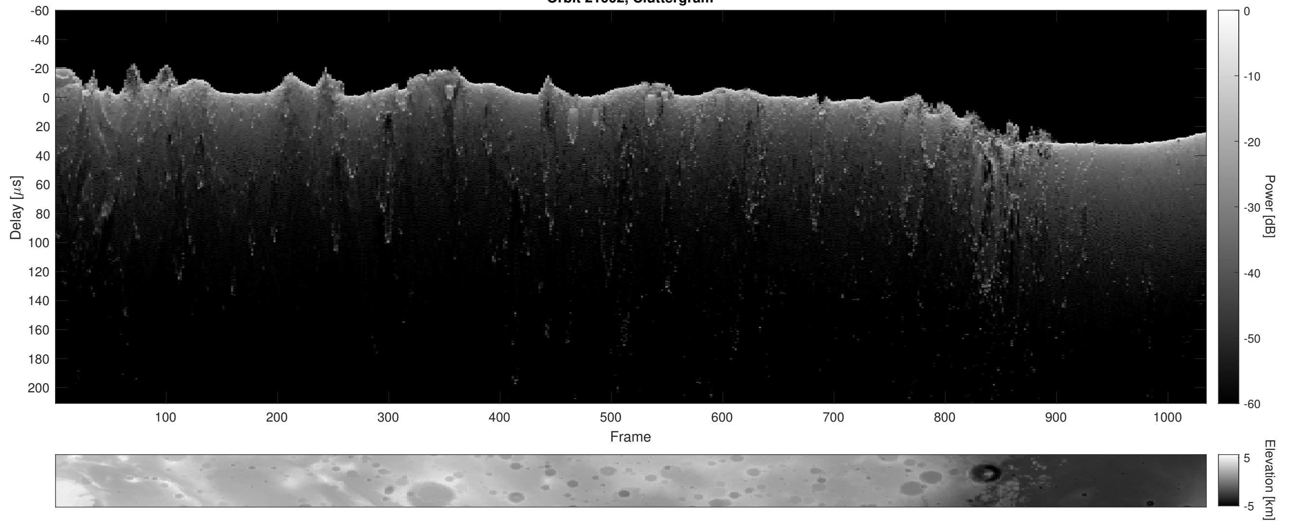
Orbit 21002, Cluttergram
