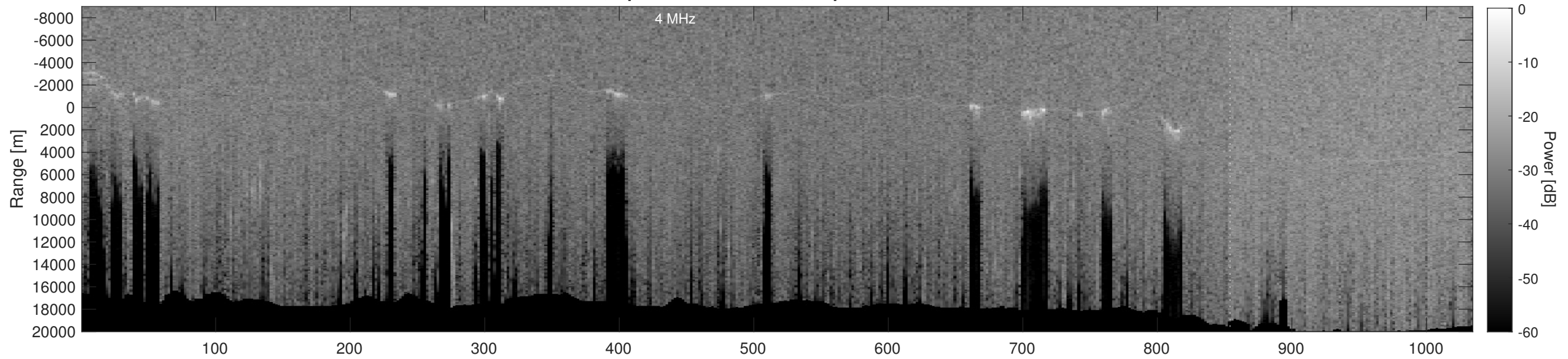
Orbit 21002, Depth-Corrected Cluttergram
