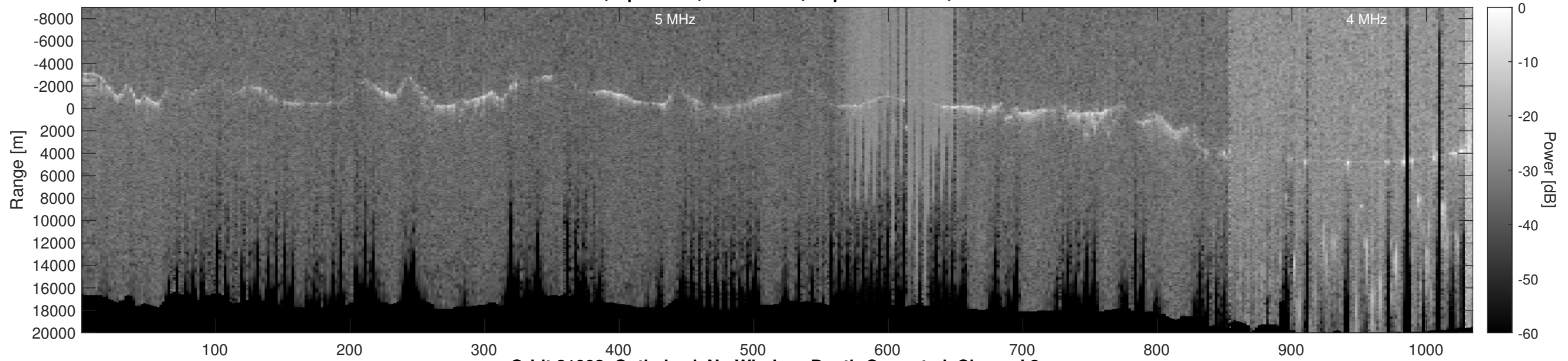
Orbit 21002, Optimized, No Window, Depth-Corrected, Channel 2
